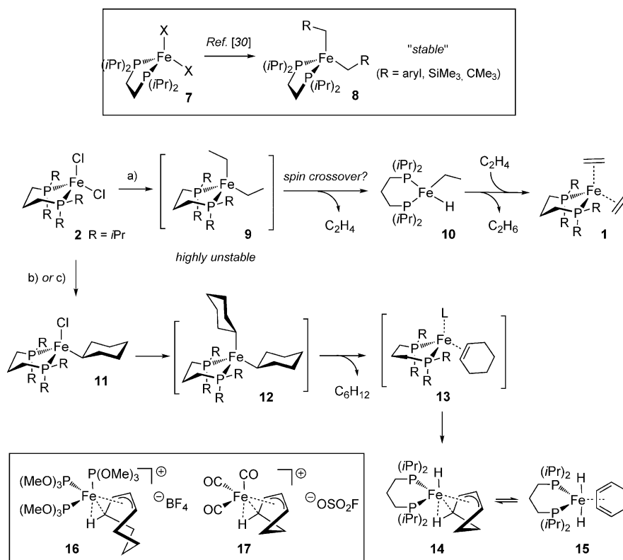
Scheme 3. a) EtMgBr, THF, ethylene, -5^{\circ}\text{C} , 77–97%; b) C 6 H 11 MgCl (1 equiv), THF, -35^{\circ}\text{C} , 51% ( 11 ); c) C 6 H 11 MgCl (2 equiv), THF, cyclohexene (5 equiv), -30^{\circ}\text{C} , 79% ( 14/15 ).
